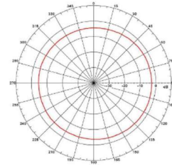
Far-field amplitude of C07+M25-1+Cable+4.5M+11 ns
